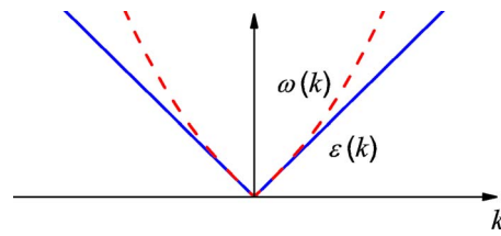
FIG. 3. (Color online) Excitation spectrum typical for BE condensates of alkaline metals.
