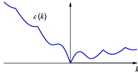
FIG. 7. (Color online) IES of tilted Hamiltonian for velocity below c_{cr} .
