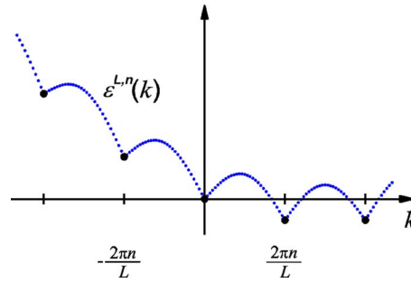
FIG. 9. (Color online) IES of “tilted Hamiltonian” in finite volume.
