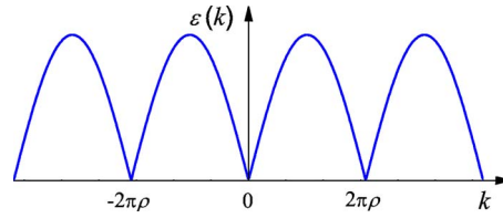
FIG. 6. (Color online) Typical IES of Bose gas in dimension d=1 .
