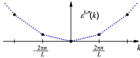
FIG. 4. (Color online) IES of free Bose gas in finite volume.
