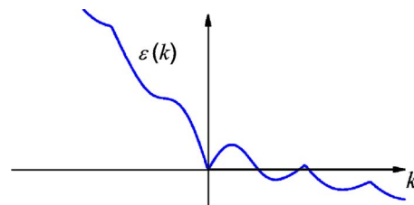
FIG. 8. (Color online) IES of tilted Hamiltonian for velocity above c_{cr} .
