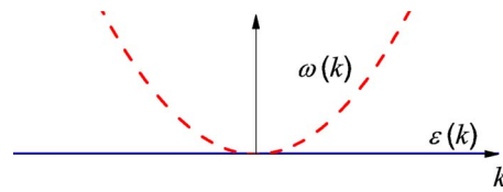
FIG. 1. (Color online) Excitation spectrum of the free Bose gas.
