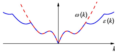
FIG. 2. (Color online) Excitation spectrum of helium IV.
