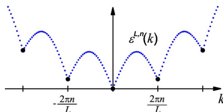
FIG. 5. (Color online) Typical IES of interacting Bose gas in finite volume.
