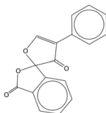
Fluorescamine
