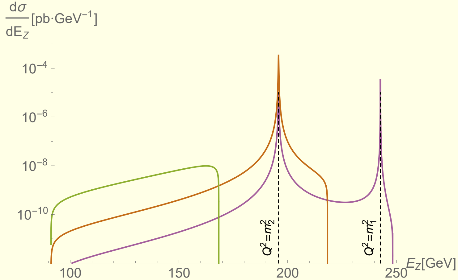
Figure 3: \frac{d\sigma}{dE_Z} for the SDM model.
