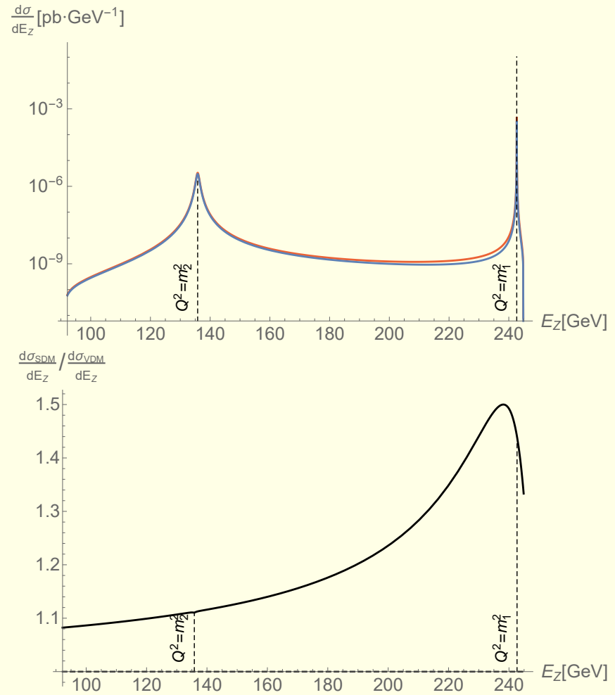
Figure 4: Two poles case: 2 \cdot m_{DM} < m_{1,2} .
