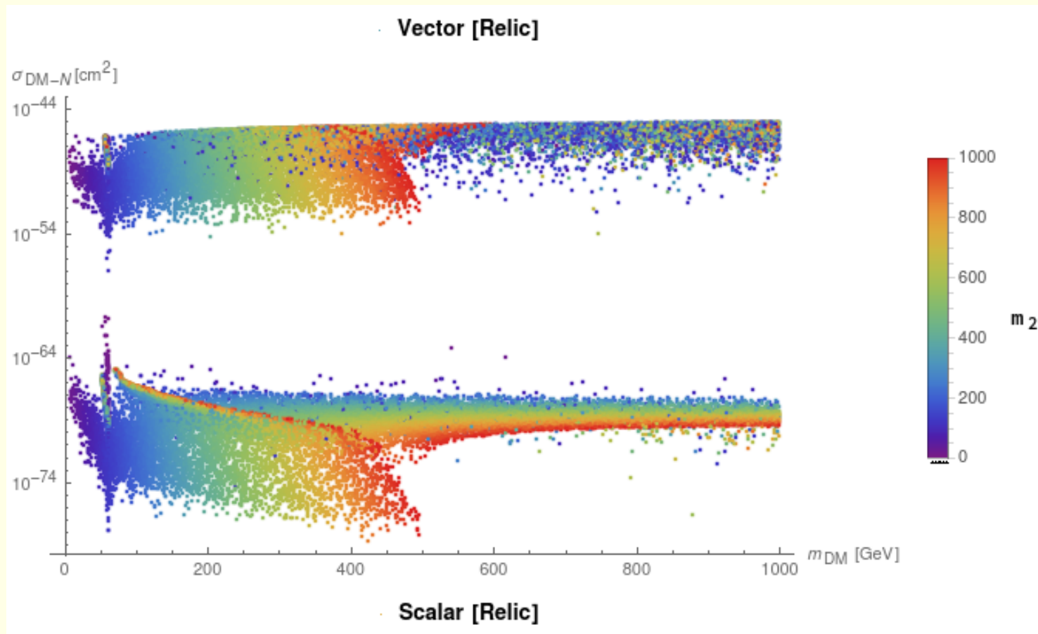
Figure 9: Dark matter-nucleon cross section versus m_{DM} colored with respect to m_2 . DM abundance is within 5\sigma of experimental value.
