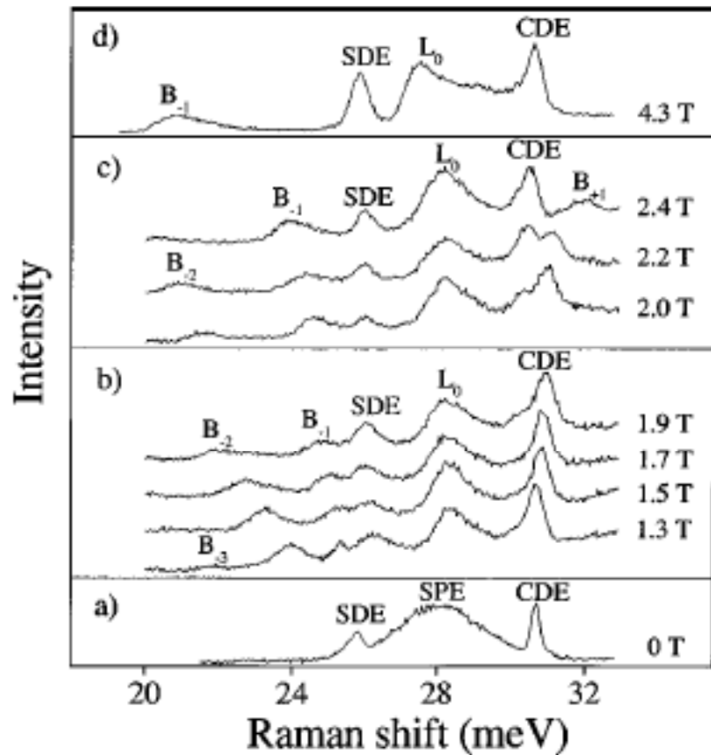
FIG. 1. Inelastic light scattering spectra of a sample with QW width of 250 Å and n_z = 6.8 \times 10^{11} \text{ cm}^{-2} measured at q = 0.4 \times 10^5 \text{ cm}^{-1} , E_L = 1.587 \text{ eV} , and different magnetic fields.
