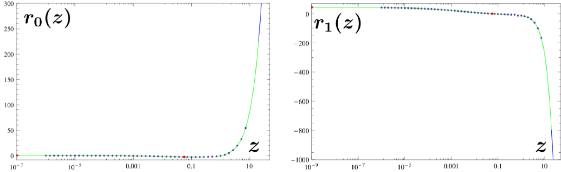
Figure 4.3: The functions r_i(z) defined in Eq. (4.16).
