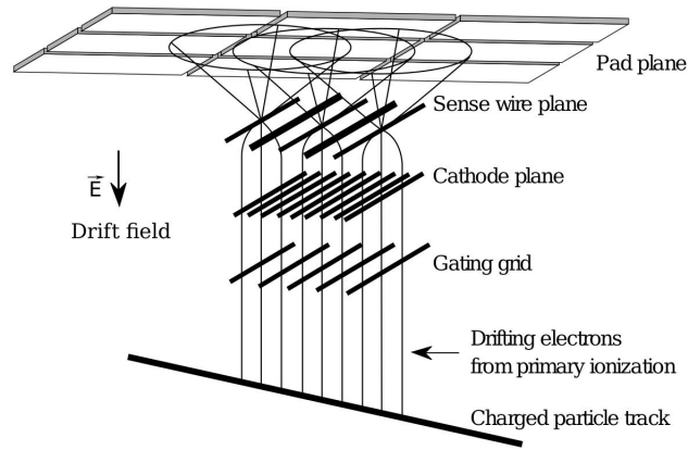
Figure 2.7: A schematic layout of the TPC readout chamber illustrating its principle of operation. Figure taken from Ref. [49].
