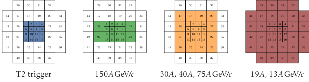
Figure 5.3: PSD modules used in the online and offline event selection. The T2 trigger is derived from the energy deposited in the central 16 modules, while the set of modules used to determine the PSD energy E_{\text{PSD}} varies with beam momentum.
