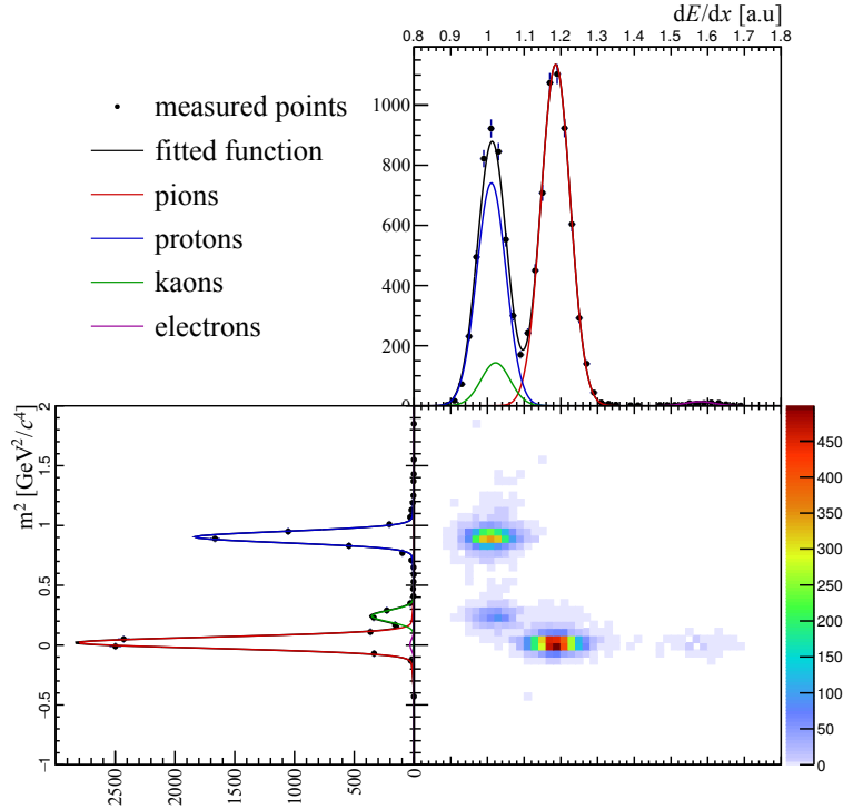
Figure 5.12: An example distribution of m^2 versus dE/dx in a single phase space bin ( 2 \text{ GeV}/c < p < 3 \text{ GeV}/c , 0.5 \text{ GeV}/c < p_T < 0.6 \text{ GeV}/c ) with fitted tof - dE/dx function for positively charged particles measured in Ar+Sc collisions at 30A GeV.
