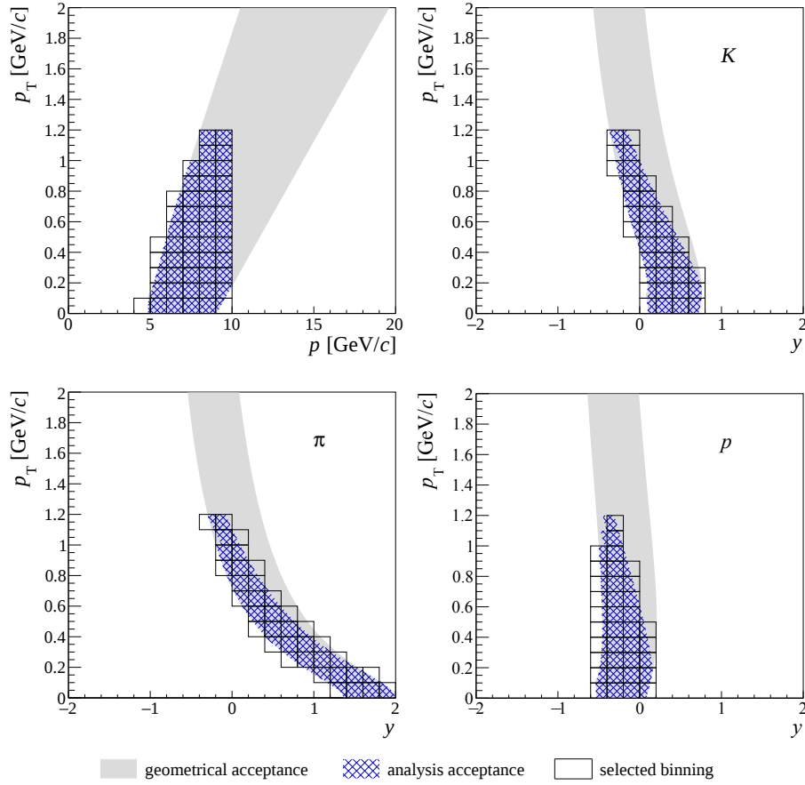
Figure 5.1: Example of the tof - dE/dx analysis acceptance for 150A GeV/c presented in p - p_T space (top left) and y - p_T space for kaons (top right), pions (bottom left) and protons (bottom right). Gray shaded area denotes the geometrical acceptance of the TPC-ToF detection system. Blue mesh represents region accepted for the analysis in bins defined by the solid black lines.
