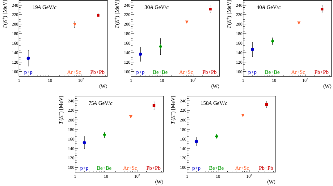
Figure 6.19: System size dependence of the inverse slope parameter T of K^+ transverse momentum spectra in mid-rapidity measured at 19A-150A GeV/c. The mean number of wounded nucleons \langle W \rangle is used as a measure of the system size. Results for p+p ([36]), Be+Be ([34]), Ar+Sc (this thesis), and Pb+Pb ([32, 88]) are shown.
