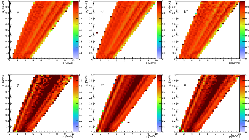
Figure 5.15: MC correction factors for inefficient (<50%) ToF pixels for Ar+Sc collisions at 75A GeV/c.
