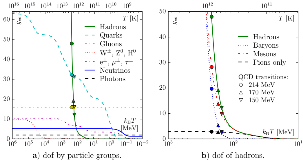
Figure 5. Panel (a) shows the contribution to the effective degrees of freedom (dof) for energy density from all particle groups. The drop in each group's g_{*\epsilon} value corresponds to ongoing annihilations of particles at that temperature. Panel (b) shows the total hadron contribution (green solid curve) to g_{*\epsilon} around the QCD phase transition temperature. We have further divided this into a baryon part (blue dotted curve) and a meson part (red dash-dotted curve). We have also plotted the pions specifically (black dashed curve), as they are the main hadronic contributor to g_{*\epsilon} at low temperatures. The two plots clearly show how fast the hadronic contribution increases at temperatures beyond 100 MeV. In both panels, we have marked the contribution to g_{*\epsilon} from hadrons, baryons, and mesons, at the three transition values of 214 MeV ( \circ symbols), 170 MeV ( \triangle symbols), and 150 MeV ( \nabla symbols), respectively.
