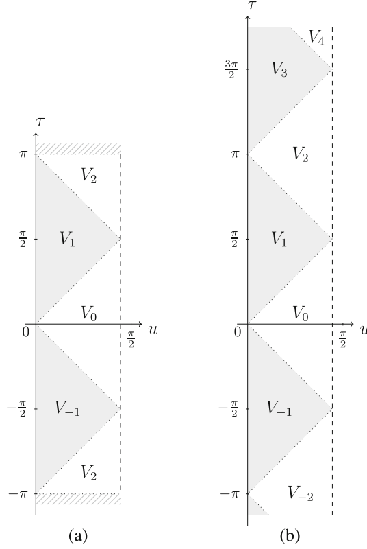
FIGURE 2. (a) Anti-de Sitter space in the coordinates u \in [0, \frac{\pi}{2}[ and \tau \in ]-\pi, \pi] from (6.5) and its partition into the regions V_0 , V_2 , V_1 and V_{-1} . Each point represents a d-2 -sphere of the coordinates \Omega . The lines \tau = \pi and \tau = -\pi are glued together, reflecting the cyclicity of time. An observer can reach spatial infinity ( u = \frac{\pi}{2} , indicated by the dashed line) in finite time, which makes it necessary to impose boundary conditions when solving the Cauchy problem for certain masses, see Sect. 6.3.4. (b) The universal cover of anti-de Sitter space in the same coordinates, where, however, \tau ranges over all of \mathbb{R} , removing the cyclicity of time. The boundary at u = \frac{\pi}{2} is still present
