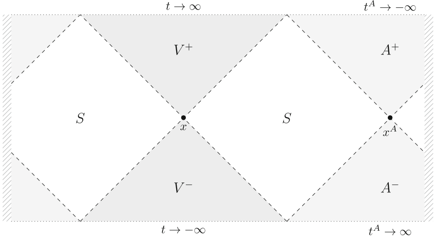
FIGURE 1. Conformal diagram of de Sitter space with the reference point x and the regions V^\pm := \{Z(x, x') > 1 \mid t(x, x') \gtrless 0\} , A^\pm := \{Z(x, x') < -1 \mid t(x^A, x') \gtrless 0\} and S := \{|Z(x, x')| < 1\} . The left and right sides of the diagram are glued together, and each point represents a d-2 -sphere
