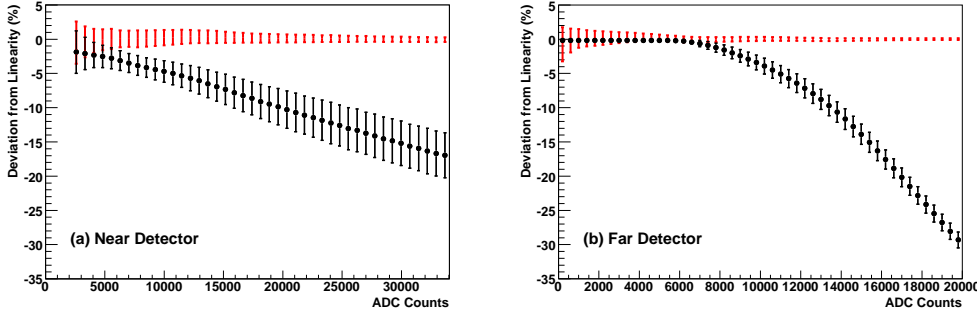
Fig. 33. Nonlinearity calibration of near and far detector instrumentation. The intrinsic nonlinearity of PMT response (circles) and its residual after calibration (error bars only) are shown for the near (a) and far (b) detectors. The error bars depict the rms spread of channels in each detector. For scale, a minimum ionizing particle normal to the plane will generate roughly 500-600 ADCs of charge each detector. A single photoelectron is roughly 75 ADCs (Far) or 100 ADCs (Near).
