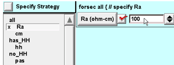
Figure 1.22. Assigning values to the biophysical parameters. Toggling Specify Strategy off shows a list of the names of the subsets that are part of the strategy. Beneath each subset are the names of the mechanisms that are associated with it. Clicking on a mechanism brings up a set of controls in the right panel for displaying and adjusting the parameters of the mechanism.
