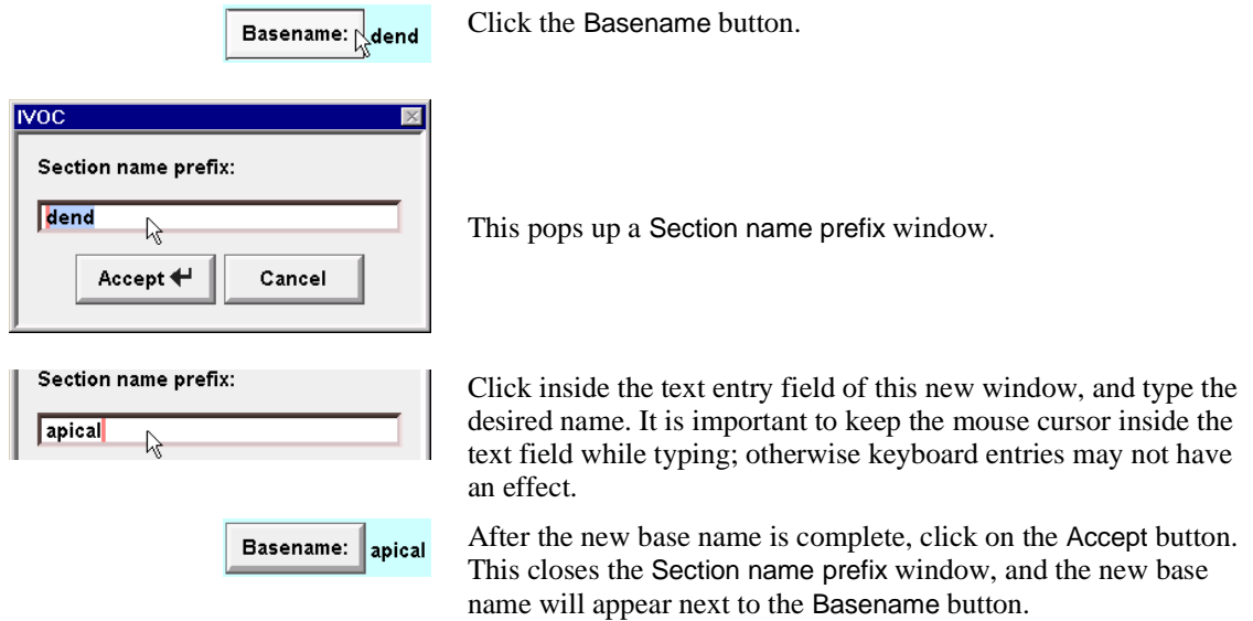
Figure 1.11. Preparing to change the name of a section. Each section we created was automatically given a name based on "dend." To change these names, we must first change the base name as shown here.
