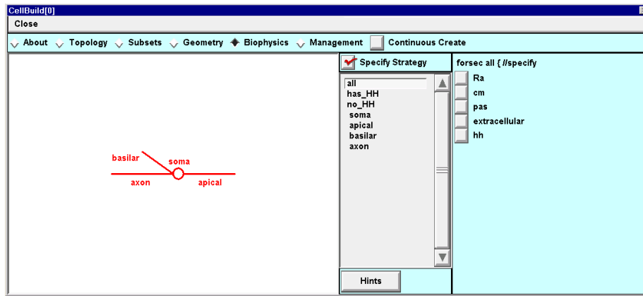
Figure 1.20. The Biophysics page, ready for specification of strategy. The right panel shows the mechanisms that are available to be inserted into our model. For this simple example, the number of mechanisms is deliberately small; adding new mechanisms is covered in Chapter 9: How to expand NEURON's library of mechanisms .
