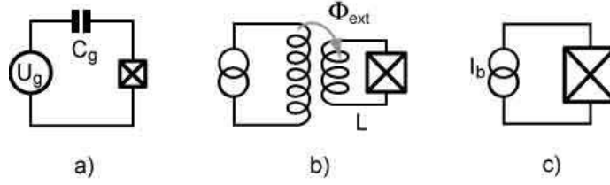
Figure 4: The three basic superconducting qubits. a) Cooper pair box (prototypal charge qubit), b) RF-SQUID (prototypal flux qubit) and c) current-biased junction (prototypal phase qubit). The charge qubit and the flux qubit requires small junctions fabricated with e-beam lithography while the phase qubit can be fabricated with conventional optical lithography.
